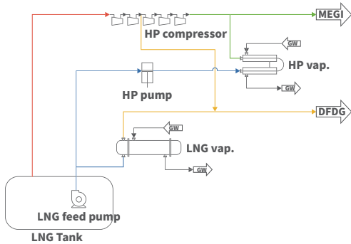
PFD - HP/LP with HP Comp.
