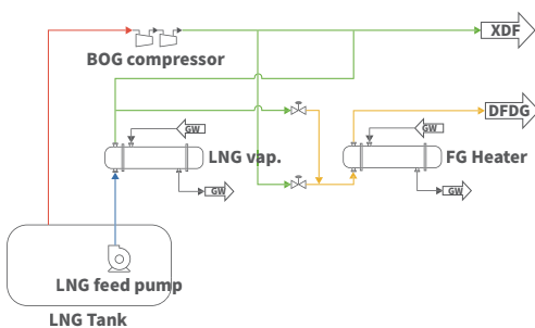
PFD - LP with BOG Comp.
