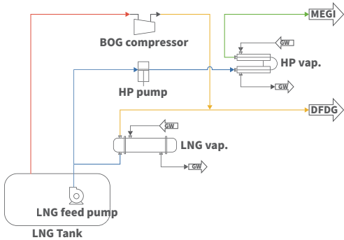
PFD - LP with BOG Comp.
